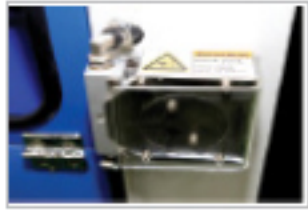
Glue Pumping Automatic glue supply with stopping sensor
